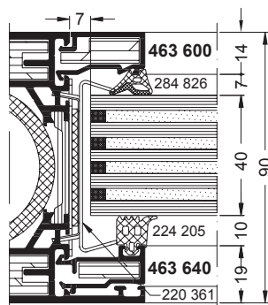
Contraflam 90-4
