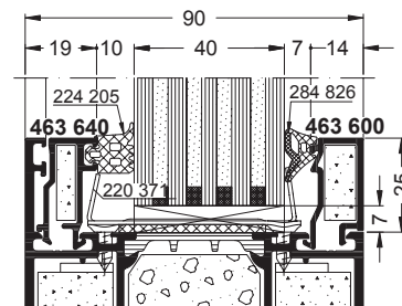
Contraflam 90-4
